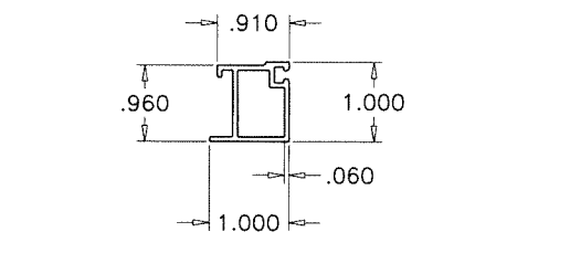
T3 TRANSOM GLASS STOP
