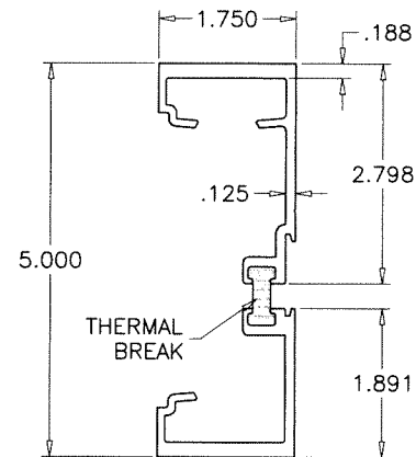
T7A TRANSOM JAMB S-8000T
