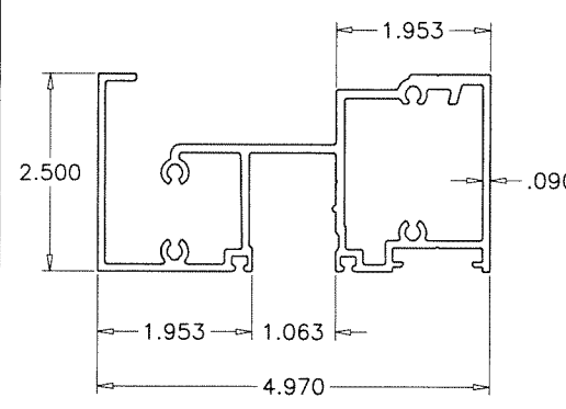
T1 TRANSOM HEADER Series 9500
