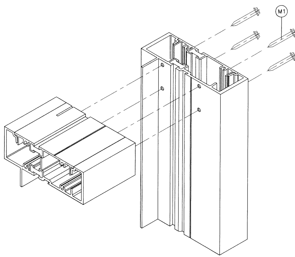
TRANSOM CORNER SERIES-8000T WINDOW WALL
