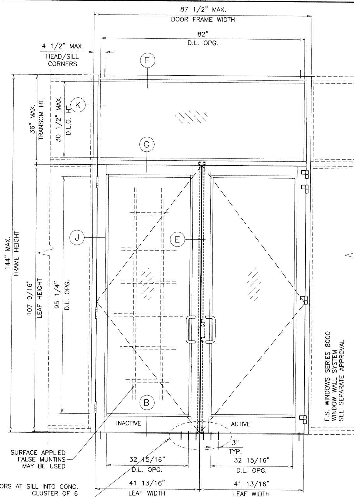
TYPICAL ELEVATION DOUBLE (O/XX) (ES-8000 TRANSOM)
