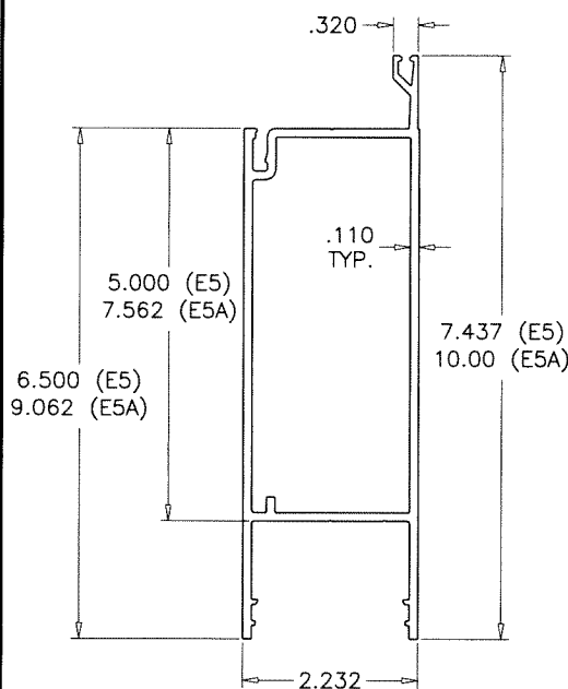
E5 STD. BOTTOM RAIL E5A HI-PROFILE BOTTOM RAIL
