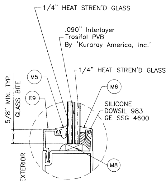
GLASS TYPE 'A.1' 9/16" OVERALL LAM. GLASS
