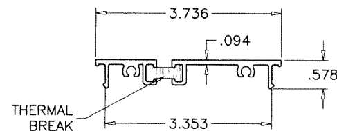
T8A TRANSOM SNAP-IN PLATE
