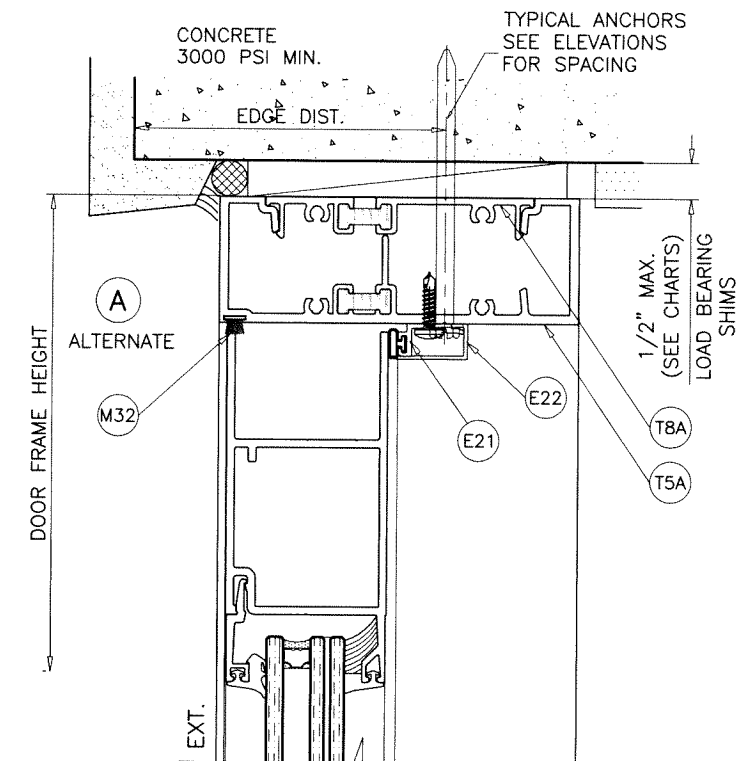
DOOR HEAD SERIES-8000T FRAME OPTION
