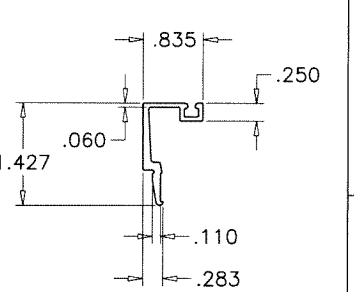
T3 TRANSOM GLASS STOP
