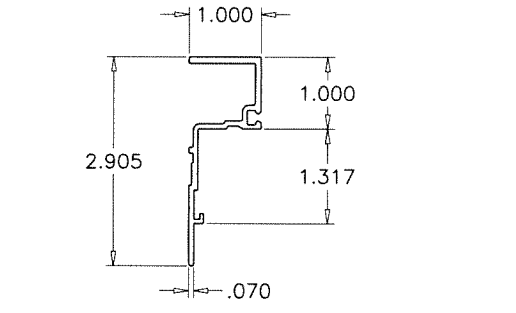
T2 TRANSOM ADAPTER
