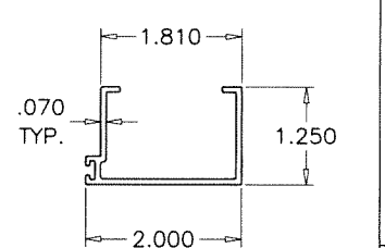
T2 TRANSOM ADAPTER
