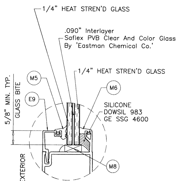
GLASS TYPE 'A.2' 9/16" OVERALL LAM. GLASS
